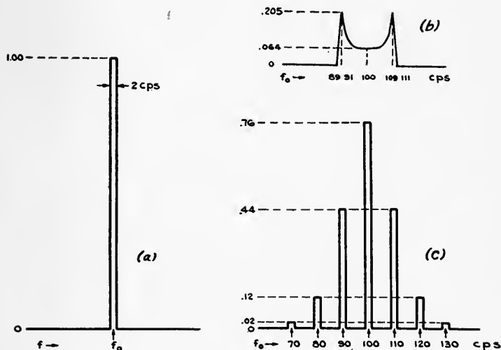
FIG. 2. Predicted transmission of warble signal: 100 cps modulated \pm 10\% ten times per second. Transmission system assumed to have characteristic a . The output signal amplitude will vary with location of f_0 . (b) Output variation as predicted by "swinging-frequency" analysis; (c) output variation predicted by "side-frequency" analysis.
